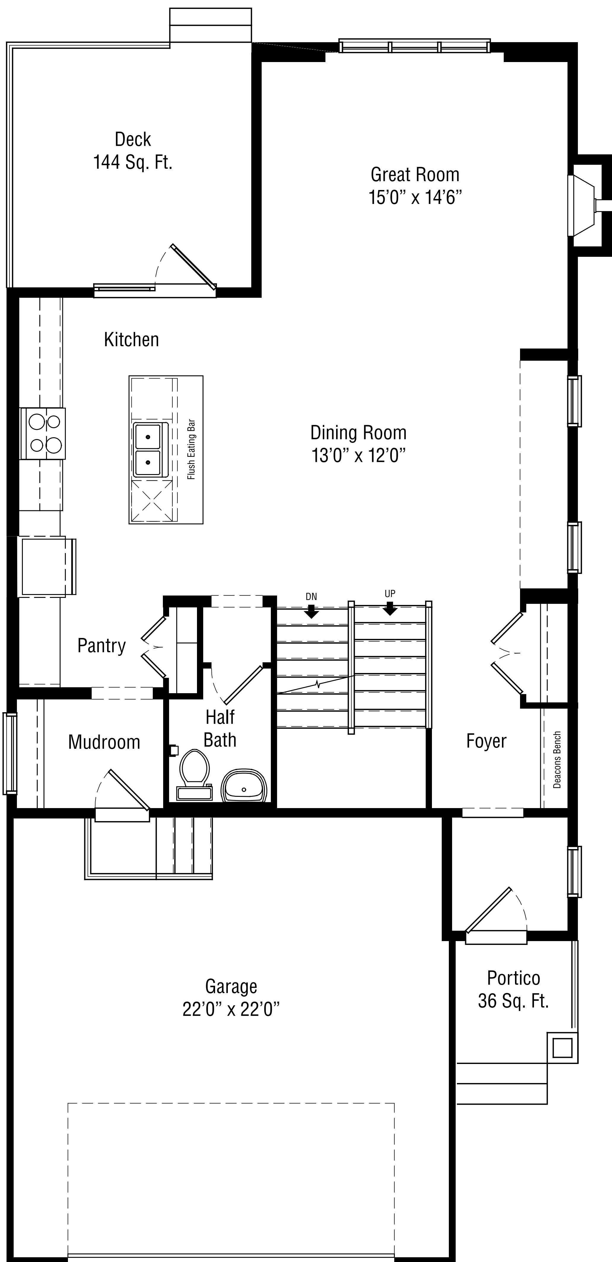
Main Floor 968 Sq. Ft.
